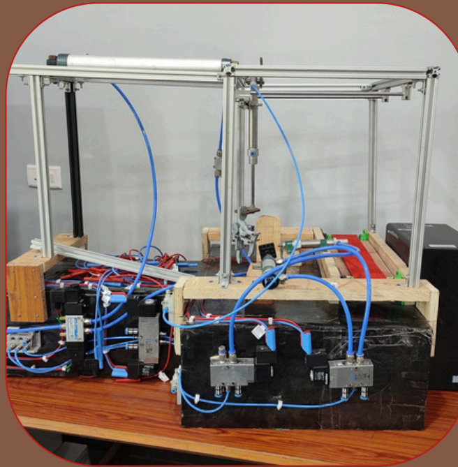
Gantry Robot
